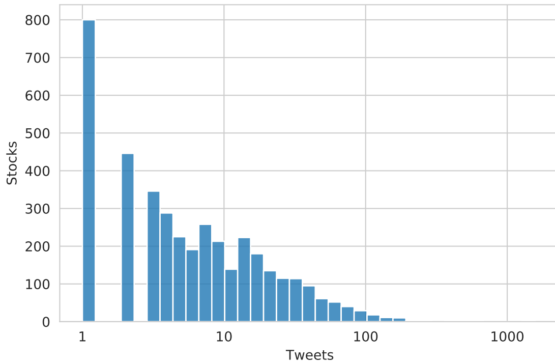
Figure A.1: The Distribution of Tweets among Stocks
